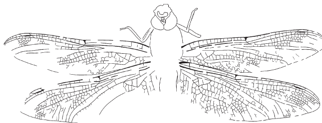
Fig. 2. Line drawing of Sophoaeschna frigida gen. et sp. nov., holotype, No. CNU-OD-NN2004015 (the scale bar is 10 mm).
