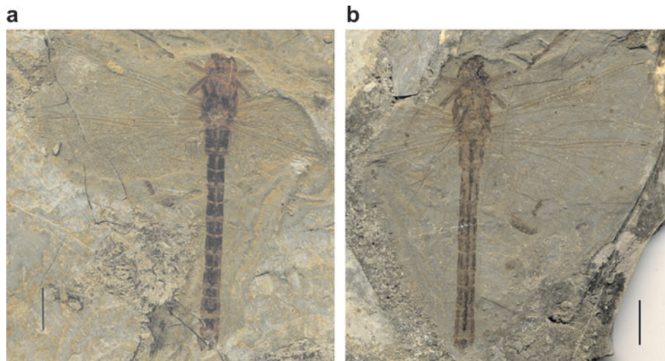
Fig. 3. Photographs of Falsisophoaeschna generalis gen. et sp. nov. (a) Holotype, No. CNU-OD-NN2004065-1, part; (b) holotype, No. CNU-OD-NN2004065-2, counterpart (the scale bar is 10 mm).
